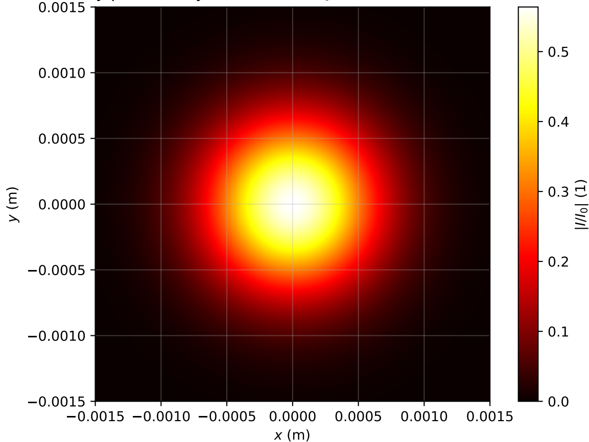
Intensity profile I(x, y, z = 1.911m)/I_0 , P_{in}=0.1P_{cr} , artificial time
